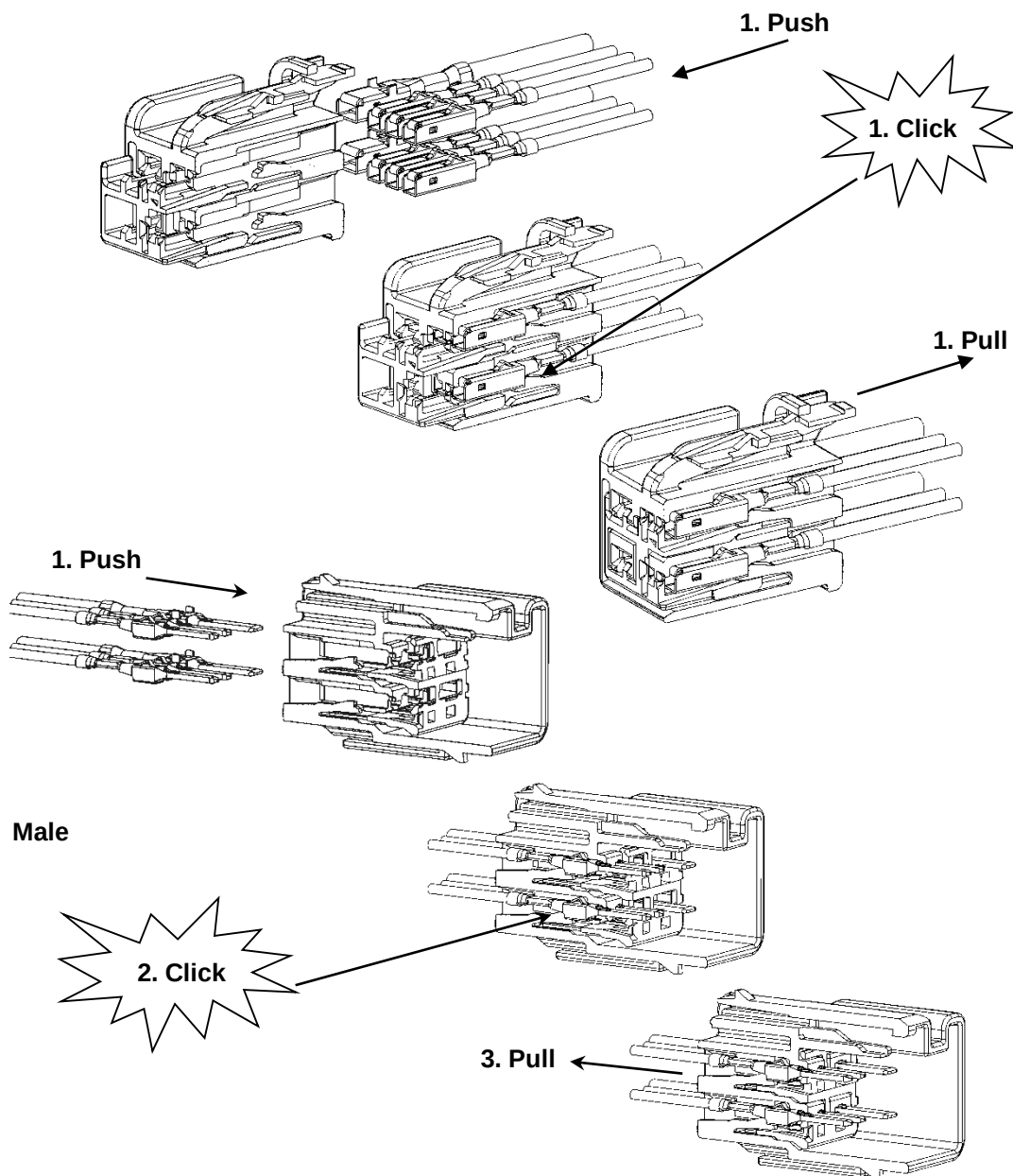
Figure 7.1. Push / Click / Pull Illustration
