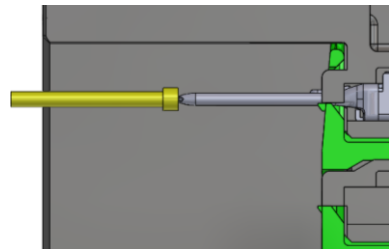
Probing 2.8mm Male Terminals
