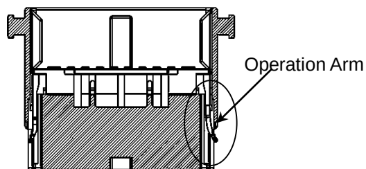
Fig. 1 Bend of Operational Arm (Unacceptable)
