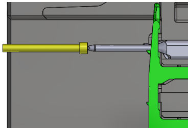
Probing 1.5mm Male Terminals
