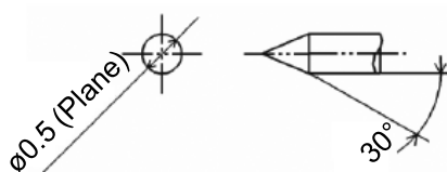
Detail of Spindle B
