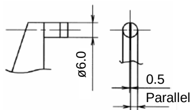
Detail of Anvil
