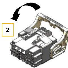
2. Pre-set position, lever rotation to mate the connectors
