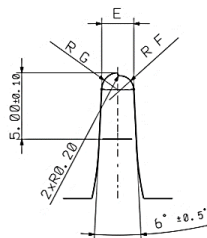
INSULATION CRIMPER
