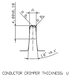
CONDUCTOR CRIMPER
