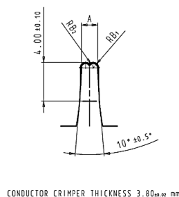
CONDUCTOR CRIMPER
