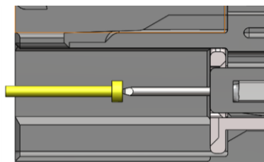
Probing 6.3mm Male Terminals
