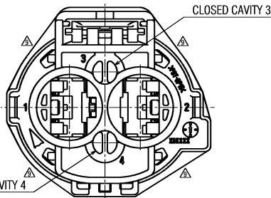
△ BACK VIEW FOR 2P CONFIGURATION
