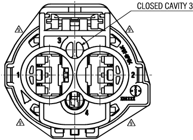
△ BACK VIEW FOR 3P CONFIGURATION
