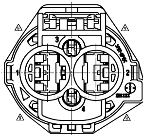
△ BACK VIEW FOR 4P CONFIGURATION
