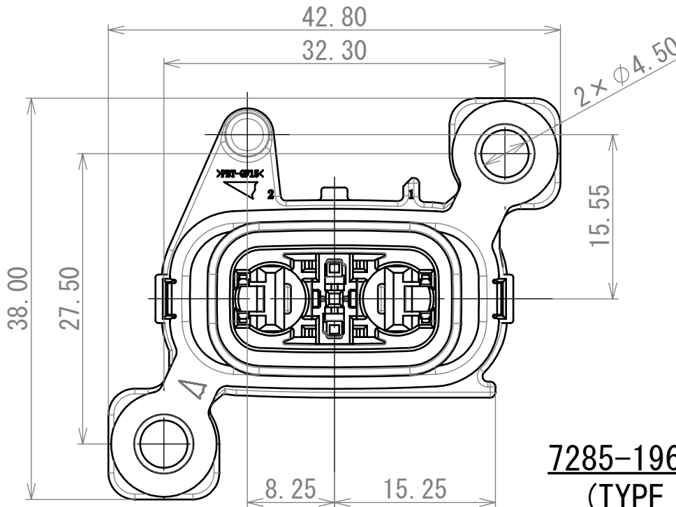
7285-1963-51 (TYPE B)
