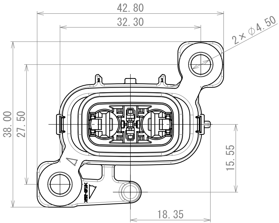
7285-1962-51 (TYPE A)
