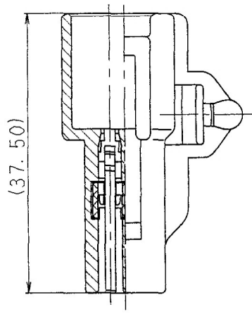
SEC. B-B
