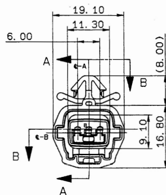
SEC. B-B
