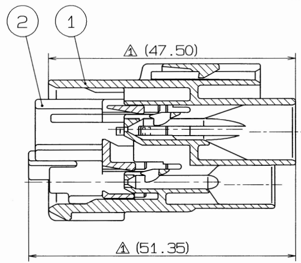
SEC. B-B
