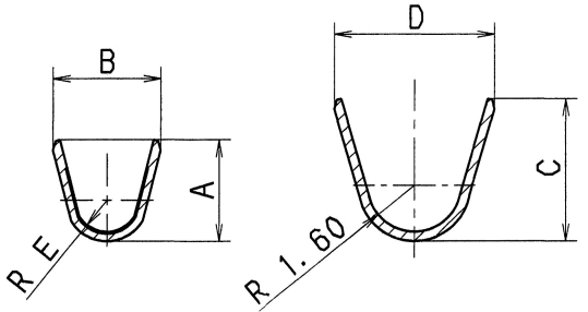
SEC. F-F SEC. G-G
