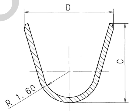
SEC. G-G (10/1)
