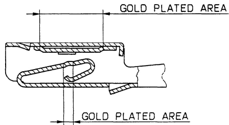
DETAIL SPLING
